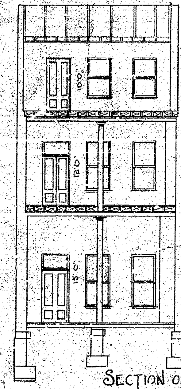
SECTION ON LINE C-D
